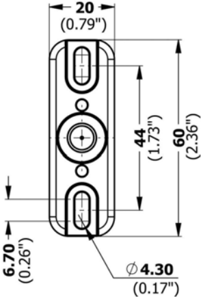
Latch
